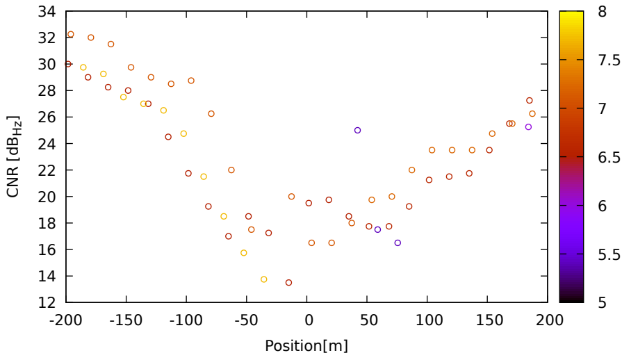
CNR vs position for E15 (E1) on XiaomiMi8 - DOY 262 jam. 2
