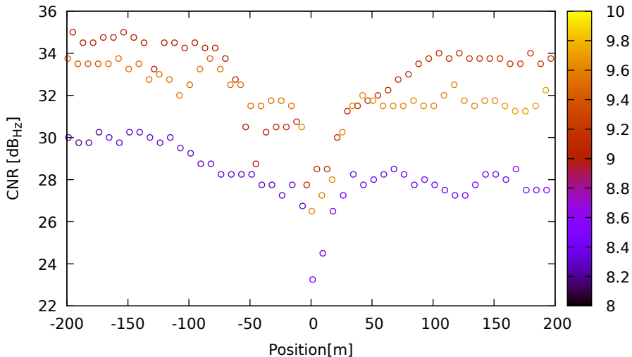
CNR vs position for E15 (E1) on XiaomiMi8 - DOY 262 jam. 3
