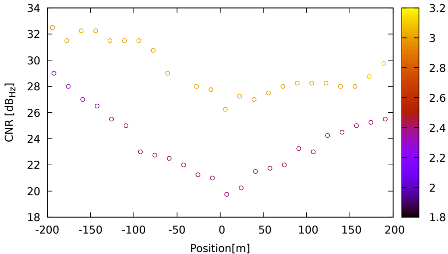
CNR vs position for E15 (E5a) on XiaomiMi8 - DOY 262 jam. 1
