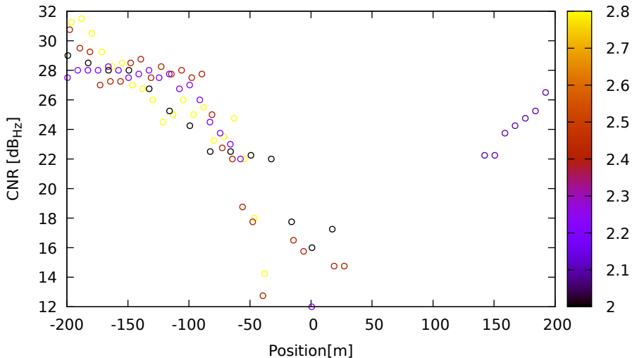
CNR vs position for E27 (E1) on XiaomiMi8 - DOY 262 jam. 2
