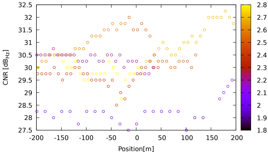
CNR vs position for E27 (E5a) on XiaomiMi8 - DOY 262 jam. 2
