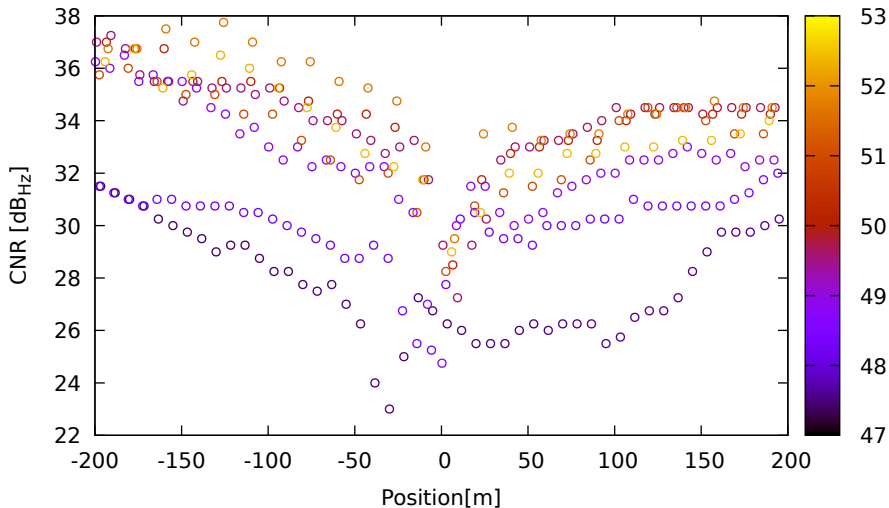
CNR vs position for E34 (E1) on XiaomiMi8 - DOY 262 jam. 1
