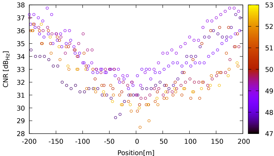
CNR vs position for E34 (E5a) on XiaomiMi8 - DOY 262 jam. 1
