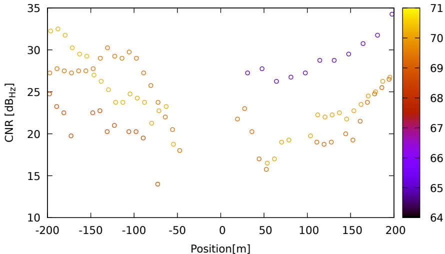
CNR vs position for E36 (E1) on XiaomiMi8 - DOY 262 jam. 2
