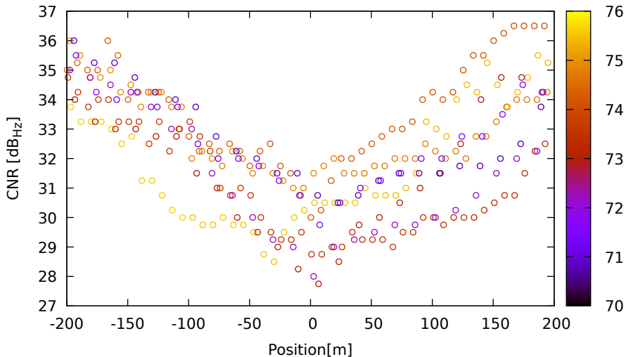
CNR vs position for E36 (E5a) on XiaomiMi8 - DOY 262 jam. 1
