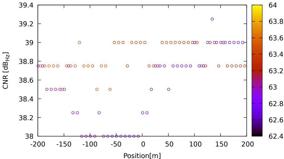
CNR vs position for E36 (E5a) on XiaomiMi8 - DOY 262 jam. 3
