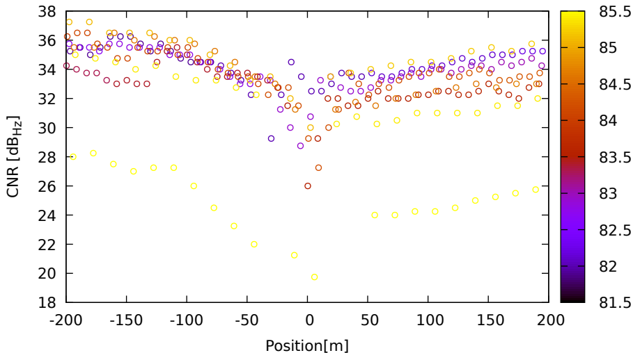
CNR vs position for G01 (L1) on XiaomiMi8 - DOY 262 jam. 1
