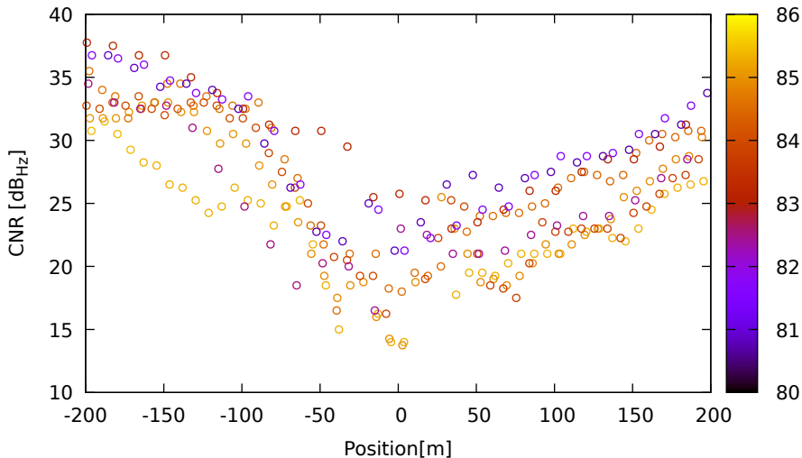
CNR vs position for G01 (L1) on XiaomiMi8 - DOY 262 jam. 2
