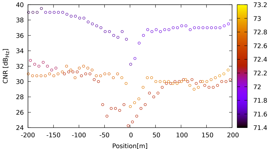
CNR vs position for G03 (L1) on XiaomiMi8 - DOY 262 jam. 3
