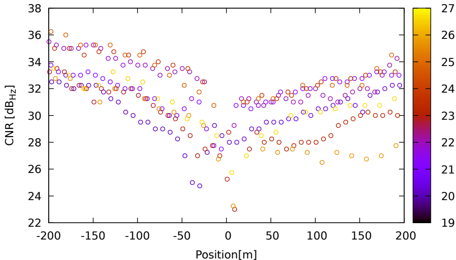
CNR vs position for G04 (L1) on XiaomiMi8 - DOY 262 jam. 1
