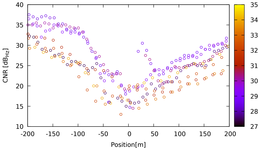
CNR vs position for G04 (L1) on XiaomiMi8 - DOY 262 jam. 2
