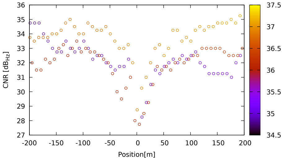
CNR vs position for G04 (L1) on XiaomiMi8 - DOY 262 jam. 3
