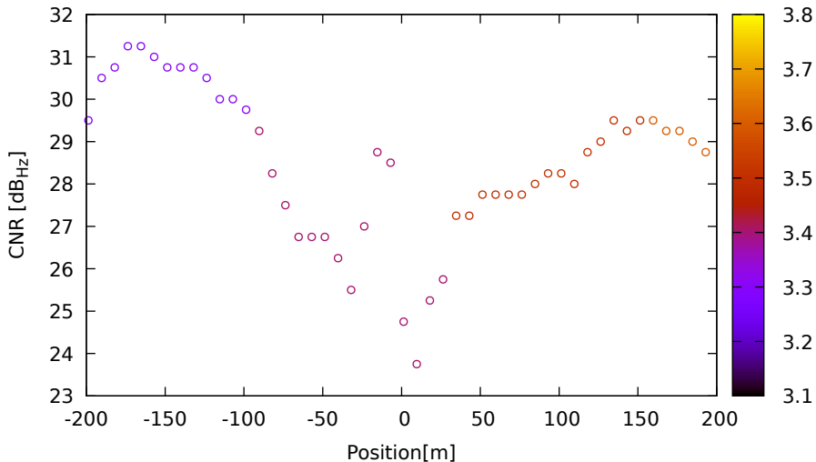
CNR vs position for G09 (L1) on XiaomiMi8 - DOY 262 jam. 3
