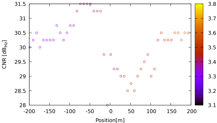
CNR vs position for G09 (L5) on XiaomiMi8 - DOY 262 jam. 3
