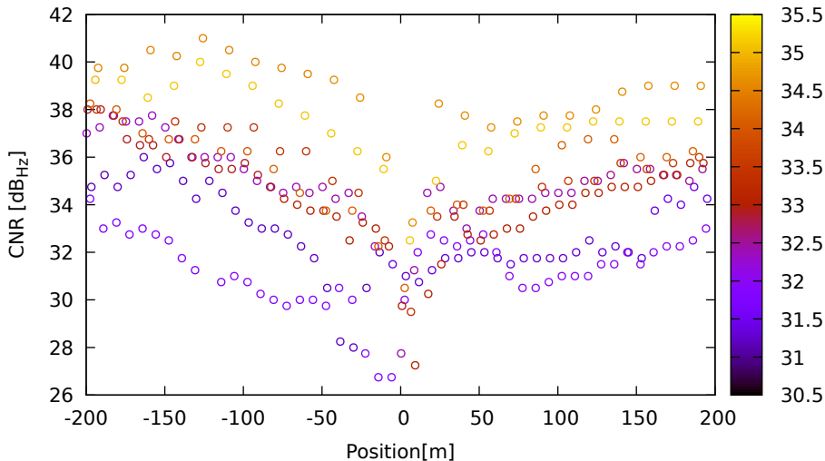
CNR vs position for G17 (L1) on XiaomiMi8 - DOY 262 jam. 1
