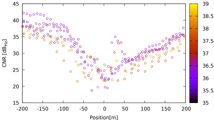
CNR vs position for G17 (L1) on XiaomiMi8 - DOY 262 jam. 2
