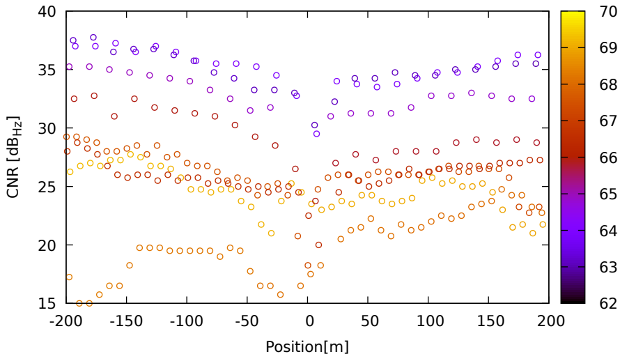
CNR vs position for G21 (L1) on XiaomiMi8 - DOY 262 jam. 1
