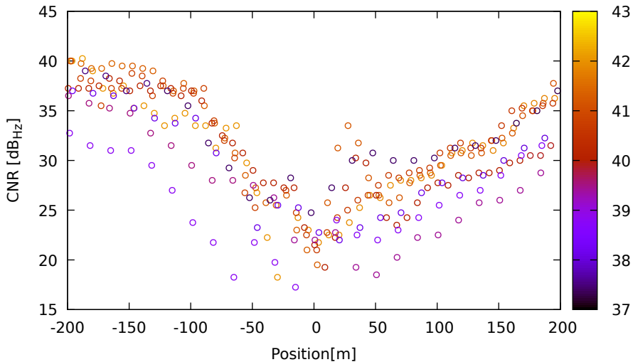
CNR vs position for G22 (L1) on XiaomiMi8 - DOY 262 jam. 2
