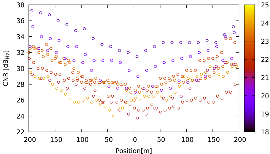
CNR vs position for G32 (L5) on XiaomiMi8 - DOY 262 jam. 1
