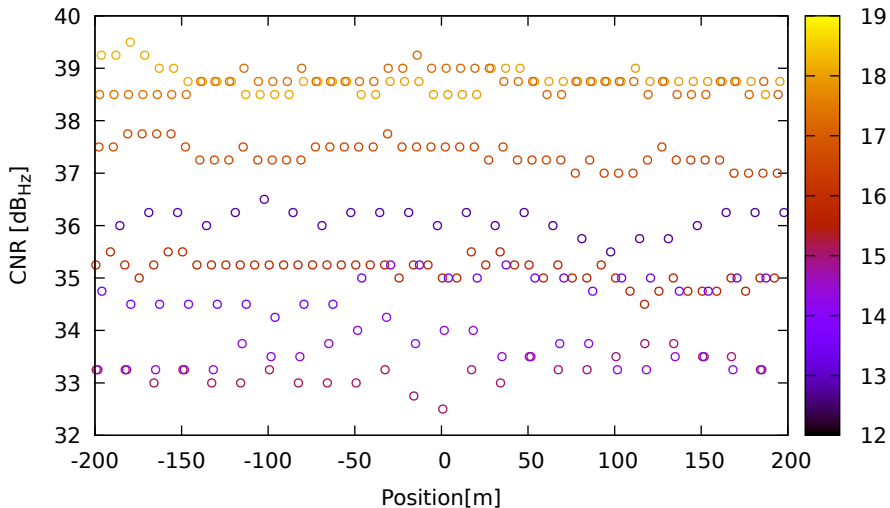
CNR vs position for G32 (L5) on XiaomiMi8 - DOY 262 jam. 2
