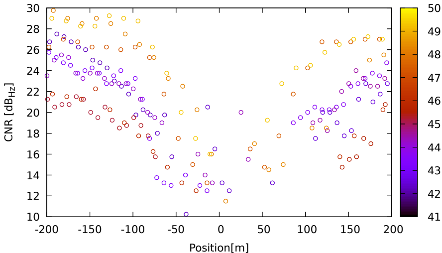
CNR vs position for R01 (G1) on XiaomiMi8 - DOY 262 jam. 1
