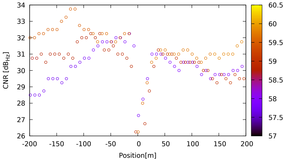
CNR vs position for R01 (G1) on XiaomiMi8 - DOY 262 jam. 3
