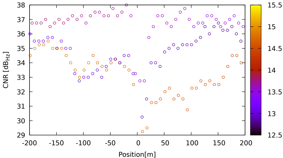
CNR vs position for R07 (G1) on XiaomiMi8 - DOY 262 jam. 3
