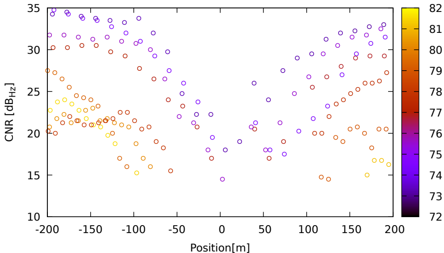
CNR vs position for R08 (G1) on XiaomiMi8 - DOY 262 jam. 1
