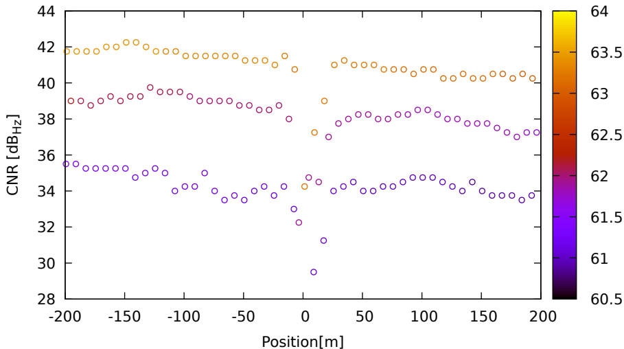
CNR vs position for R08 (G1) on XiaomiMi8 - DOY 262 jam. 3
