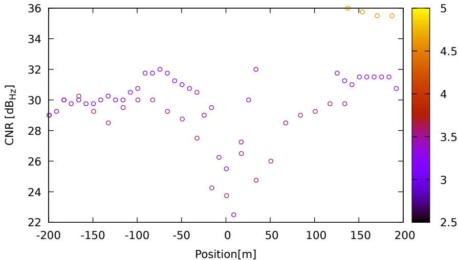
CNR vs position for R09 (G1) on XiaomiMi8 - DOY 262 jam. 2
