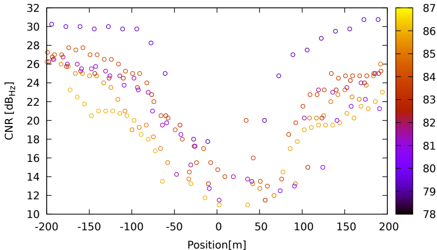
CNR vs position for R23 (G1) on XiaomiMi8 - DOY 262 jam. 1
