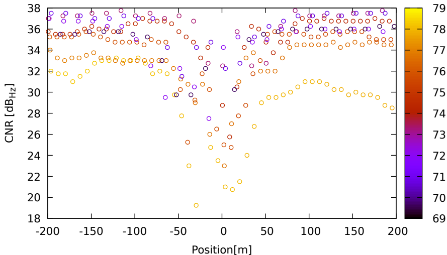
CNR vs position for R23 (G1) on XiaomiMi8 - DOY 262 jam. 2
