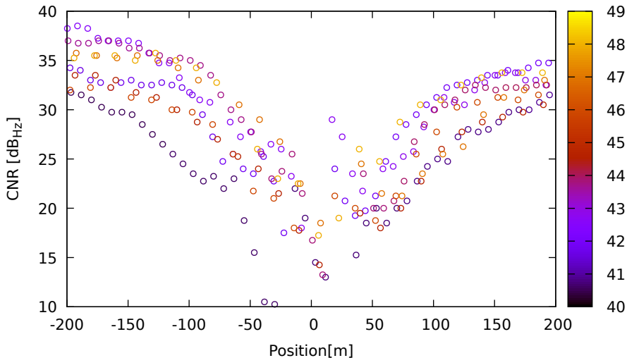
CNR vs position for R24 (G1) on XiaomiMi8 - DOY 262 jam. 1
