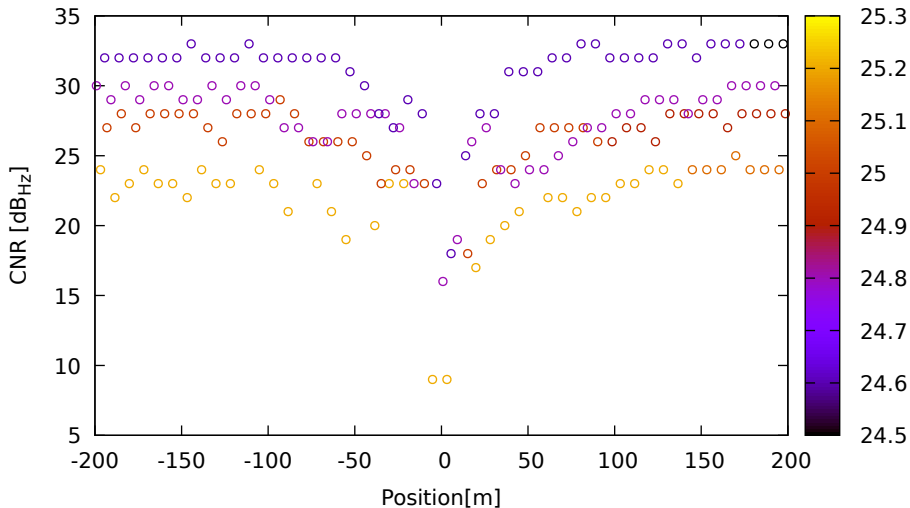
CNR vs position for C06 (B1) on HuaweiP40 - DOY 262 jam. 1
