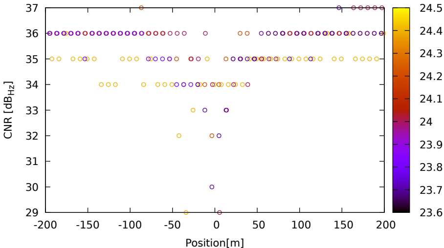
CNR vs position for C06 (B1) on HuaweiP40 - DOY 262 jam. 2
