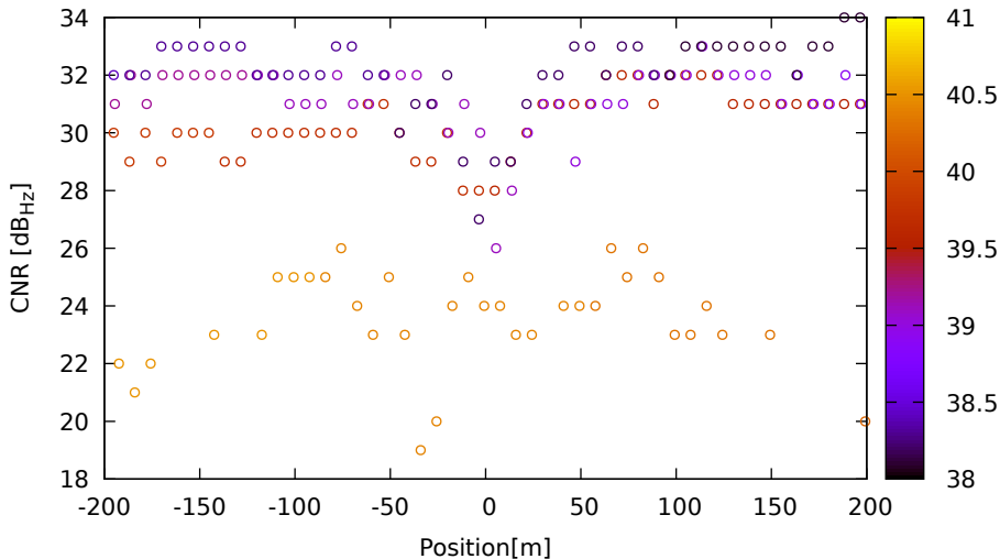
CNR vs position for C14 (B1) on HuaweiP40 - DOY 262 jam. 2
