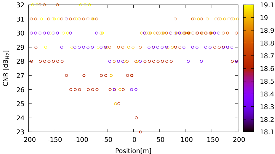
CNR vs position for C16 (B1) on HuaweiP40 - DOY 262 jam. 2
