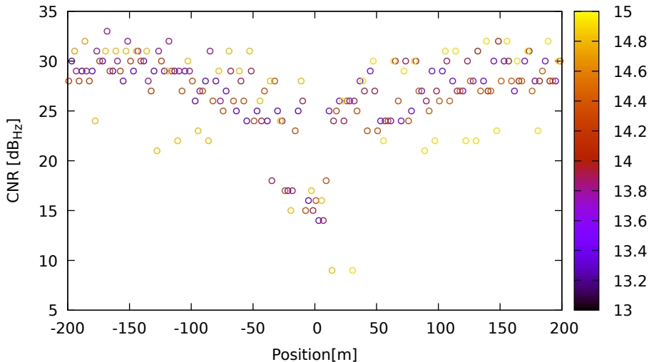
CNR vs position for C24 (B1) on HuaweiP40 - DOY 262 jam. 1
