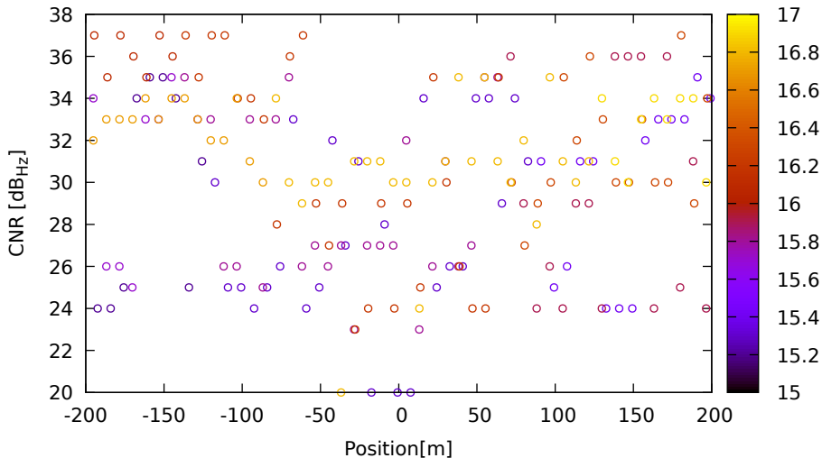
CNR vs position for C24 (B1) on HuaweiP40 - DOY 262 jam. 2
