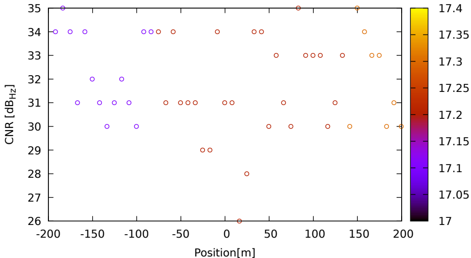
CNR vs position for C24 (B1) on HuaweiP40 - DOY 262 jam. 3
