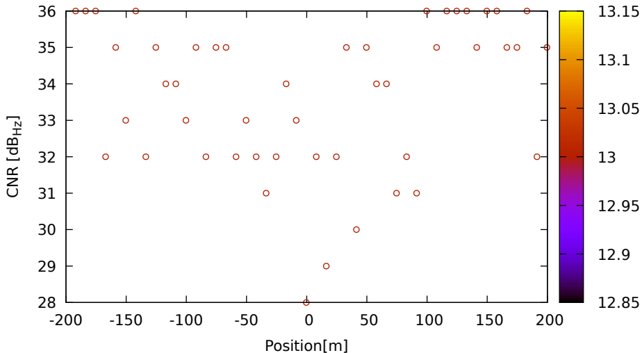
CNR vs position for C26 (B1) on HuaweiP40 - DOY 262 jam. 3
