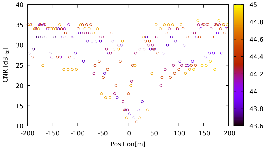
CNR vs position for C27 (B1) on HuaweiP40 - DOY 262 jam. 1
