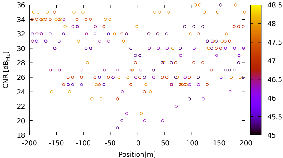
CNR vs position for C28 (B1) on HuaweiP40 - DOY 262 jam. 2
