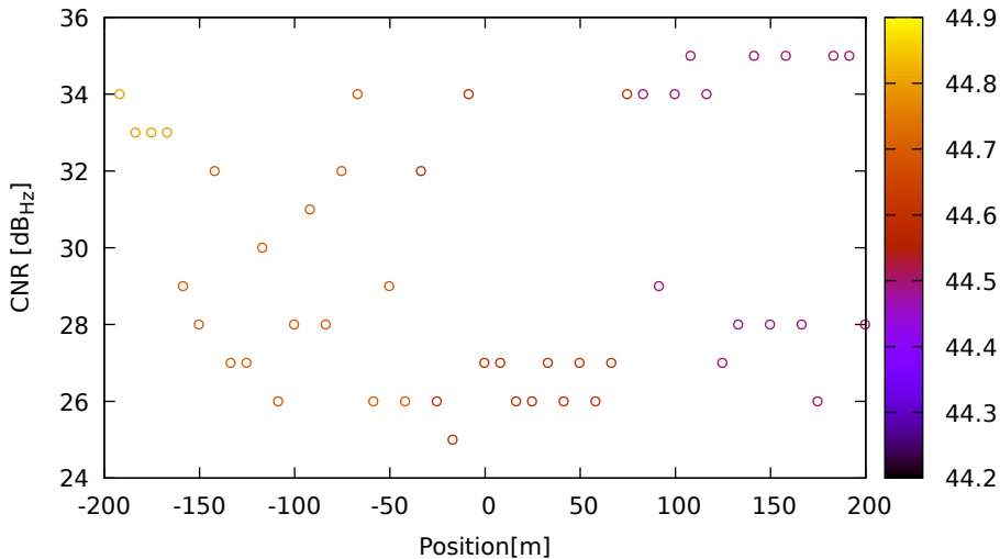
CNR vs position for C28 (B1) on HuaweiP40 - DOY 262 jam. 3
