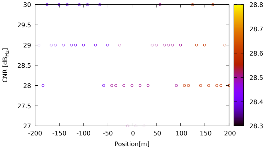
CNR vs position for E03 (E1) on HuaweiP40 - DOY 262 jam. 3
