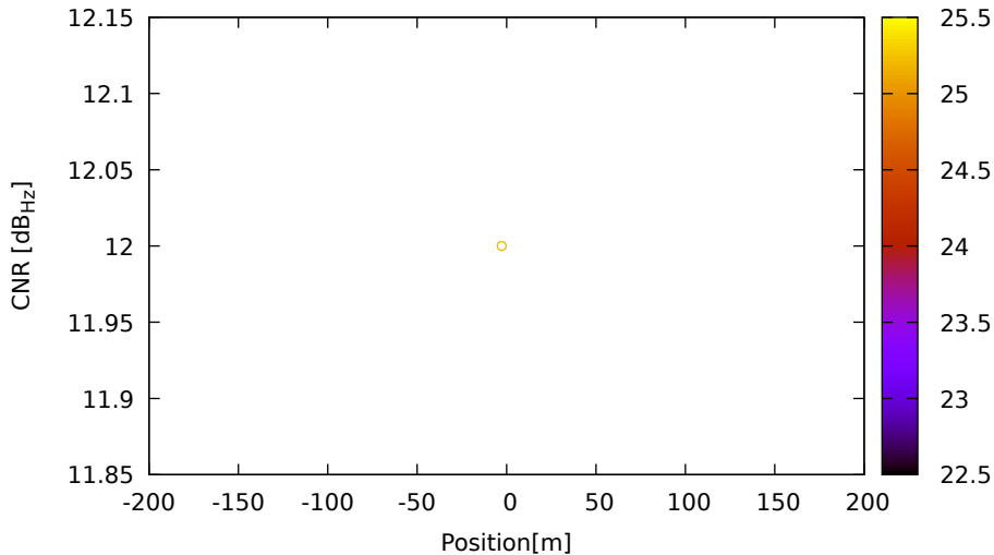
CNR vs position for E03 (E5a) on HuaweiP40 - DOY 262 jam. 1
