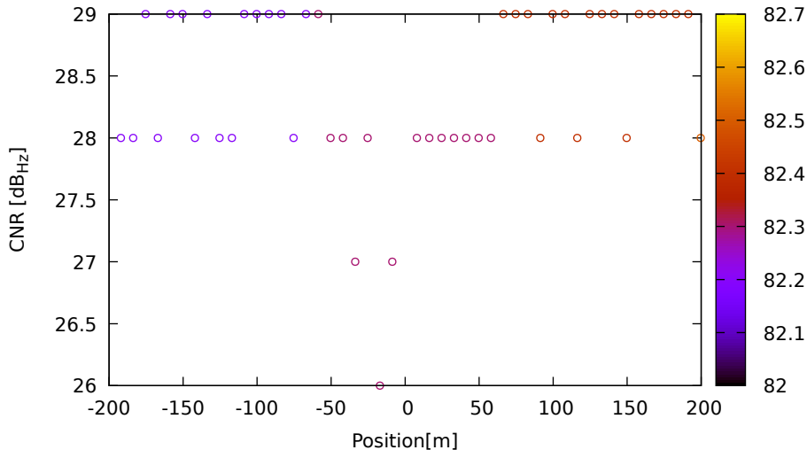
CNR vs position for E05 (E1) on HuaweiP40 - DOY 262 jam. 3
