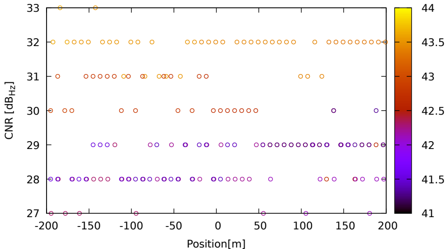
CNR vs position for E09 (E1) on HuaweiP40 - DOY 262 jam. 2
