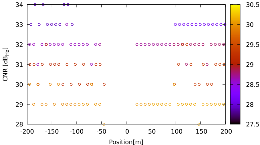
CNR vs position for E15 (E5a) on HuaweiP40 - DOY 262 jam. 2
