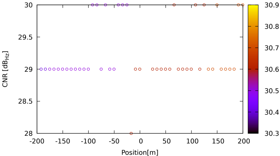
CNR vs position for E15 (E5a) on HuaweiP40 - DOY 262 jam. 3
